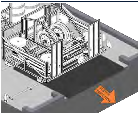
TRAILER WASHOUT CART IS HOUSED ON A FIXED HEIGHT PLATFORM AT THE EDGE OF A LOADING DOCK THAT THE TRAILER BACKS UP TO MEET.
