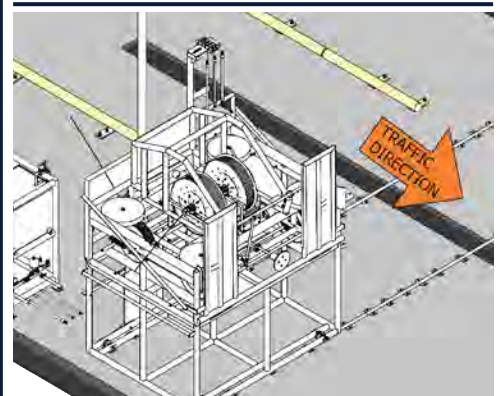
SYSTEM IS HOUSED ON A VERTICALLY ADJUSTABLE PLATFORM INSTALLED ALONG A TRACK ALLOWING IT TO MOVE LATERALLY TO MEET THE TRAILER.
