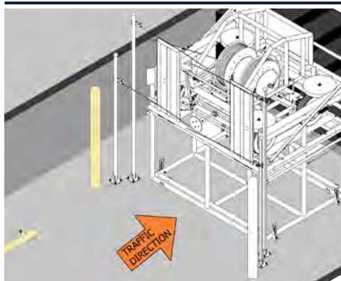
WASHOUT CART IS HOUSED ON A VERTICALLY ADJUSTABLE PLATFORM, INSTALLED IN A FIXED LOCATION THAT THE TRAILER BACKS UP TO MEET.
